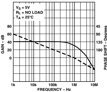
Figure 25. Open-Loop Gain & Phase vs. Frequency
