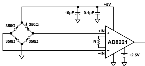
Figure 49. Precision Strain Gage
