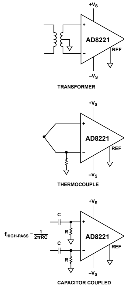
Figure 47. Creating an I BIAS Path
