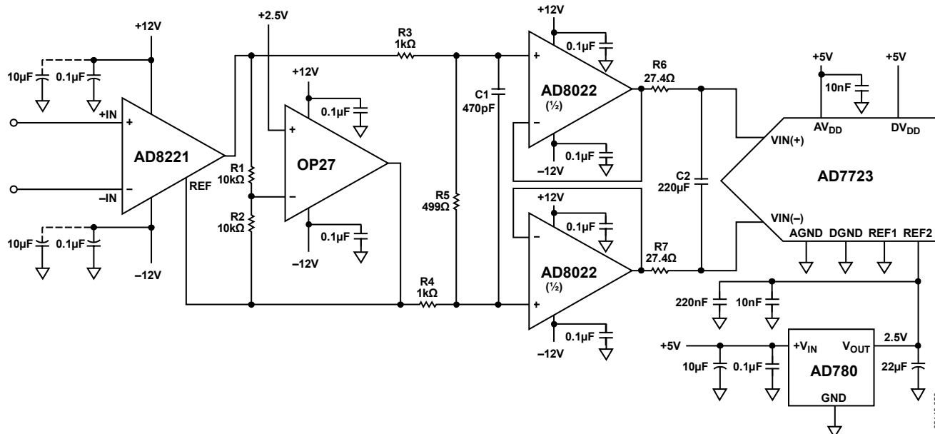
Figure 50. Interfacing to a Differential Input ADC
