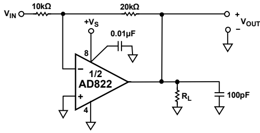
Figure 36. Gain-of-2 Inverter
