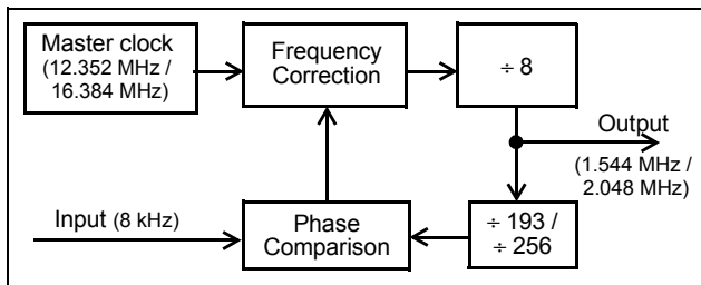
Figure 3 - DPLL Principle
