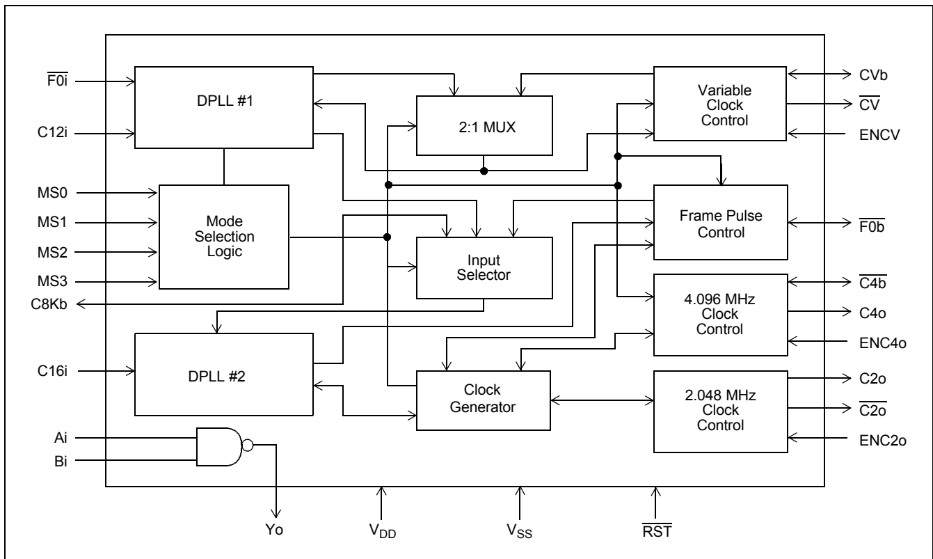
Figure 1 - Figure 1 - Functional Block Diagram
