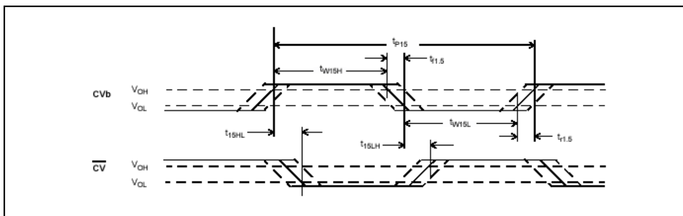
Figure 14 - Timing Information for DPLL #1 in NORMAL Mode
