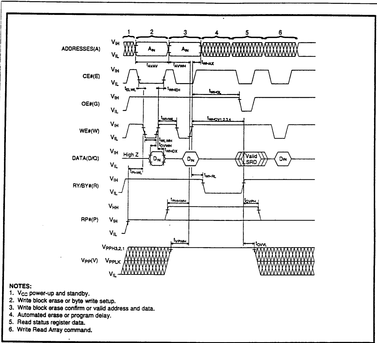
Figure 16. AC Waveform for WE#-Controlled Write Operations
