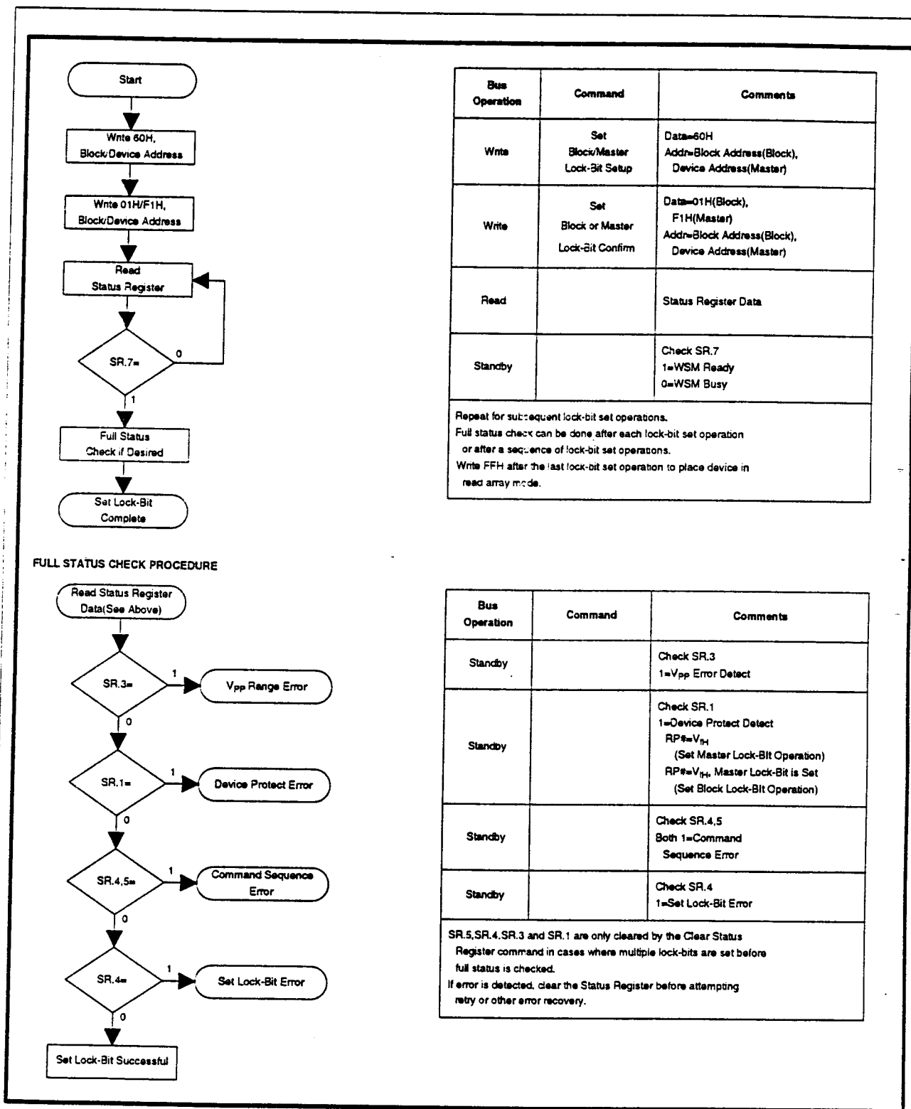
Figure 9. Set Block and Master Lock-Bit Flowchart
