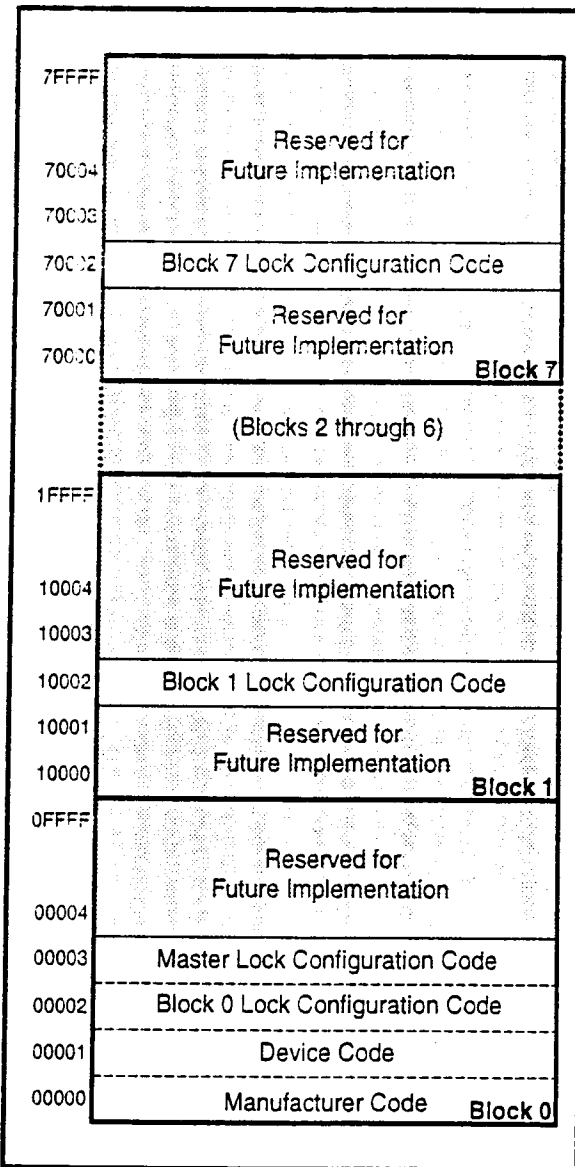
Figure 4. Device Identifier Code Memory Map
