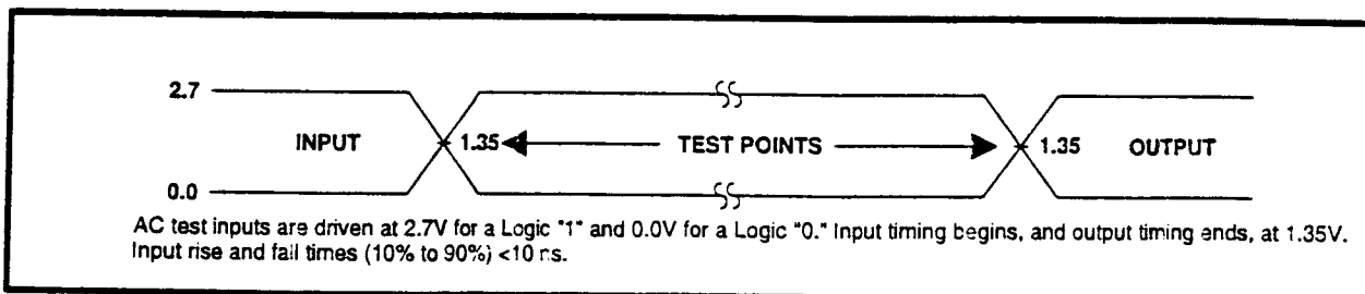
Figure 11. Transient Input/Output Reference Waveform for V_{CC}=2.7V-3.6V
