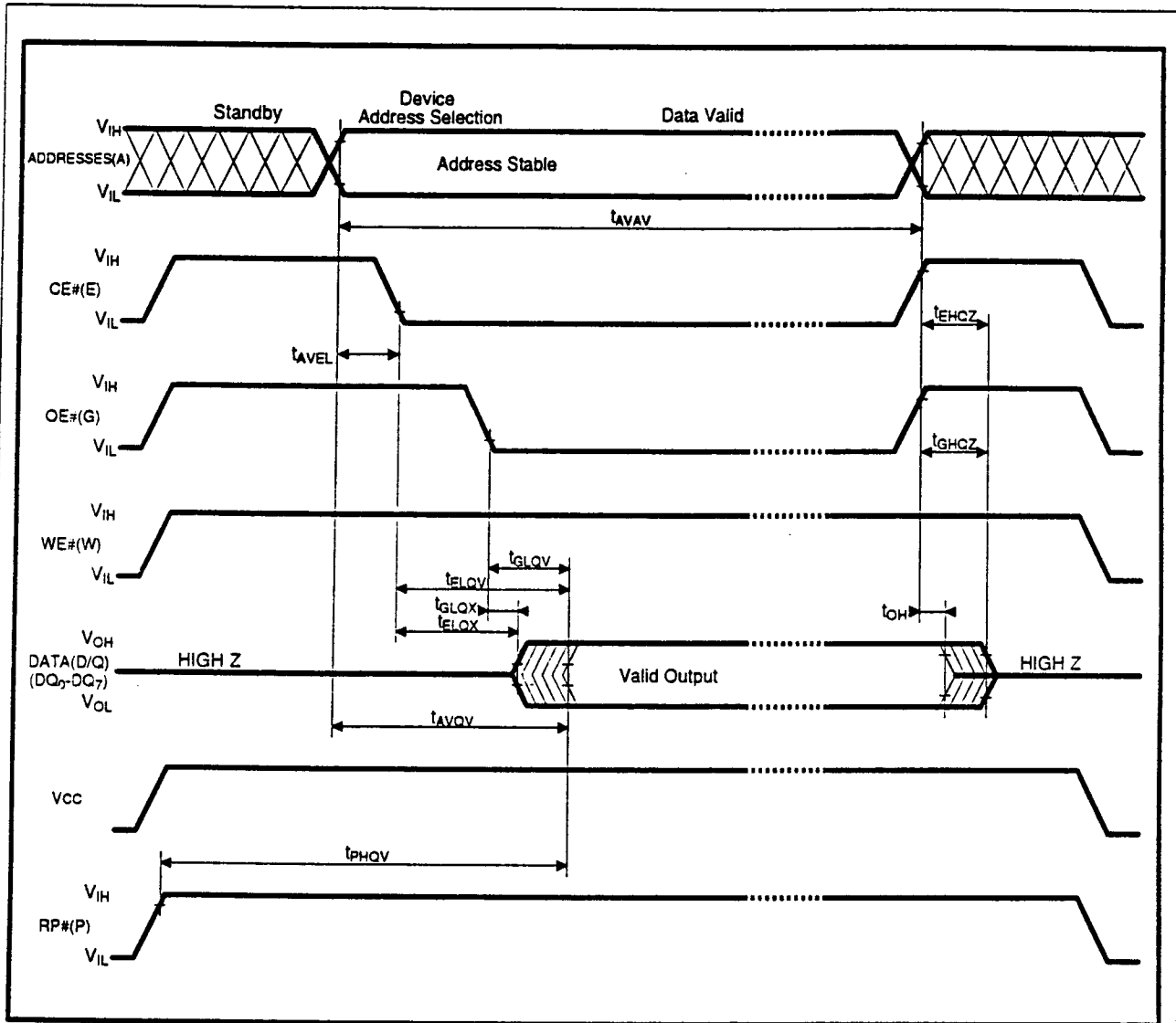
Figure 15. AC Waveform for Read Operations
