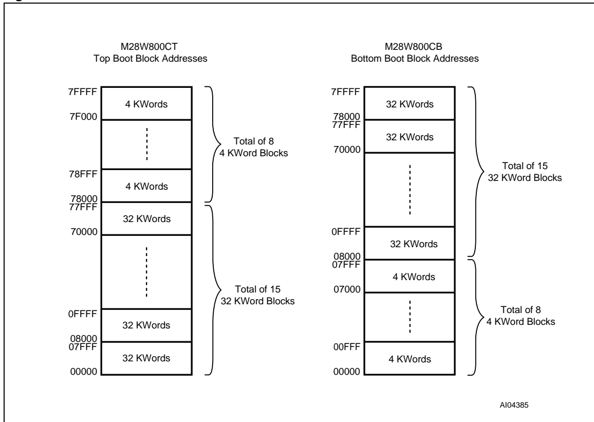
Figure 5. Block Addresses
