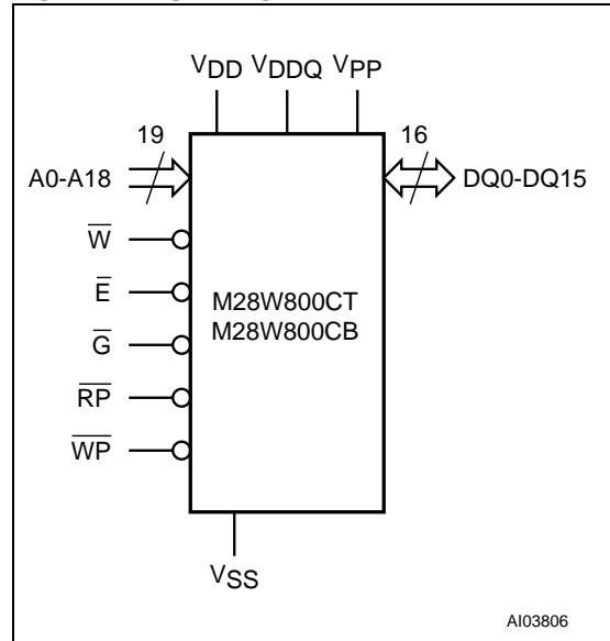
Figure 2. Logic Diagram
