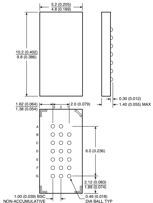
20C1, 20-ball (3 x 7 Array), 1.0 mm Pitch, 5.0 x 10.0 mm Plastic Chip-scale Ball Grid Array (CGBA) Dimensions in Millimeters and (Inches)
