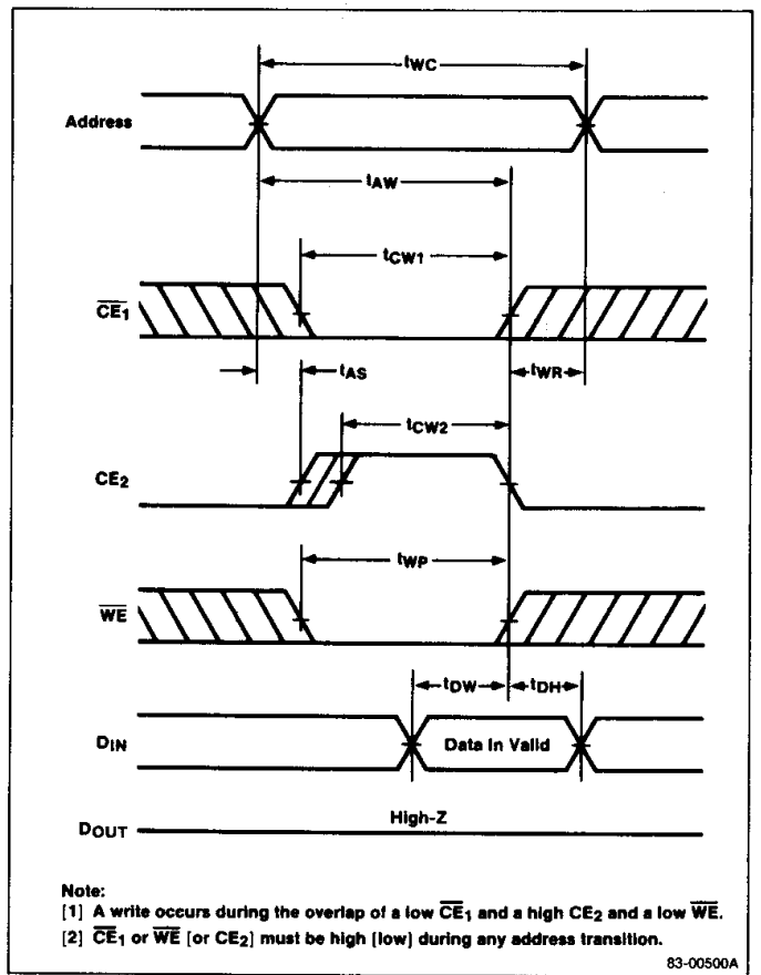
Write Cycle No. 3 ( \overline{CE}_2 -Controlled)
