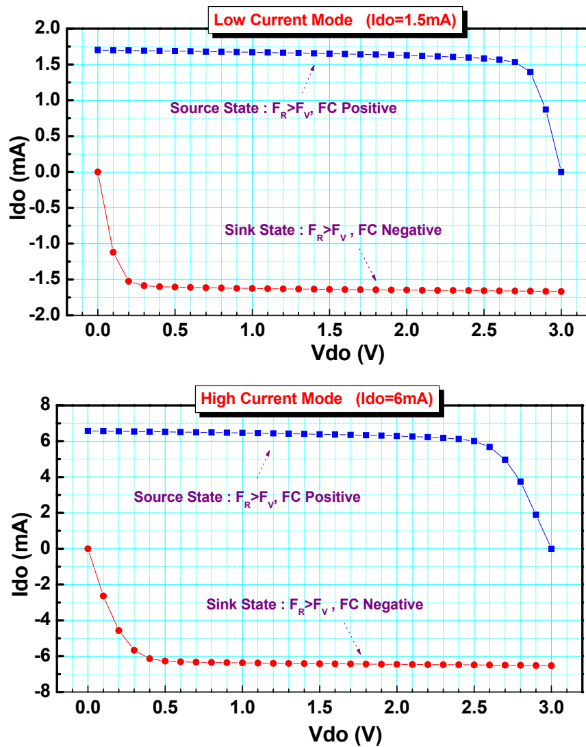
Fig. 7 – Charge pump current vs. V_{DO}
