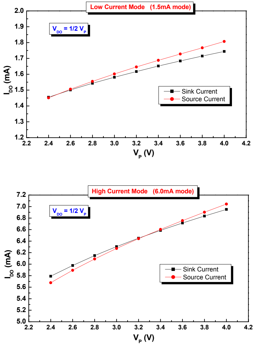
Fig. 8 – Charge pump current vs. supply voltage at V_{DO} = V_P/2
