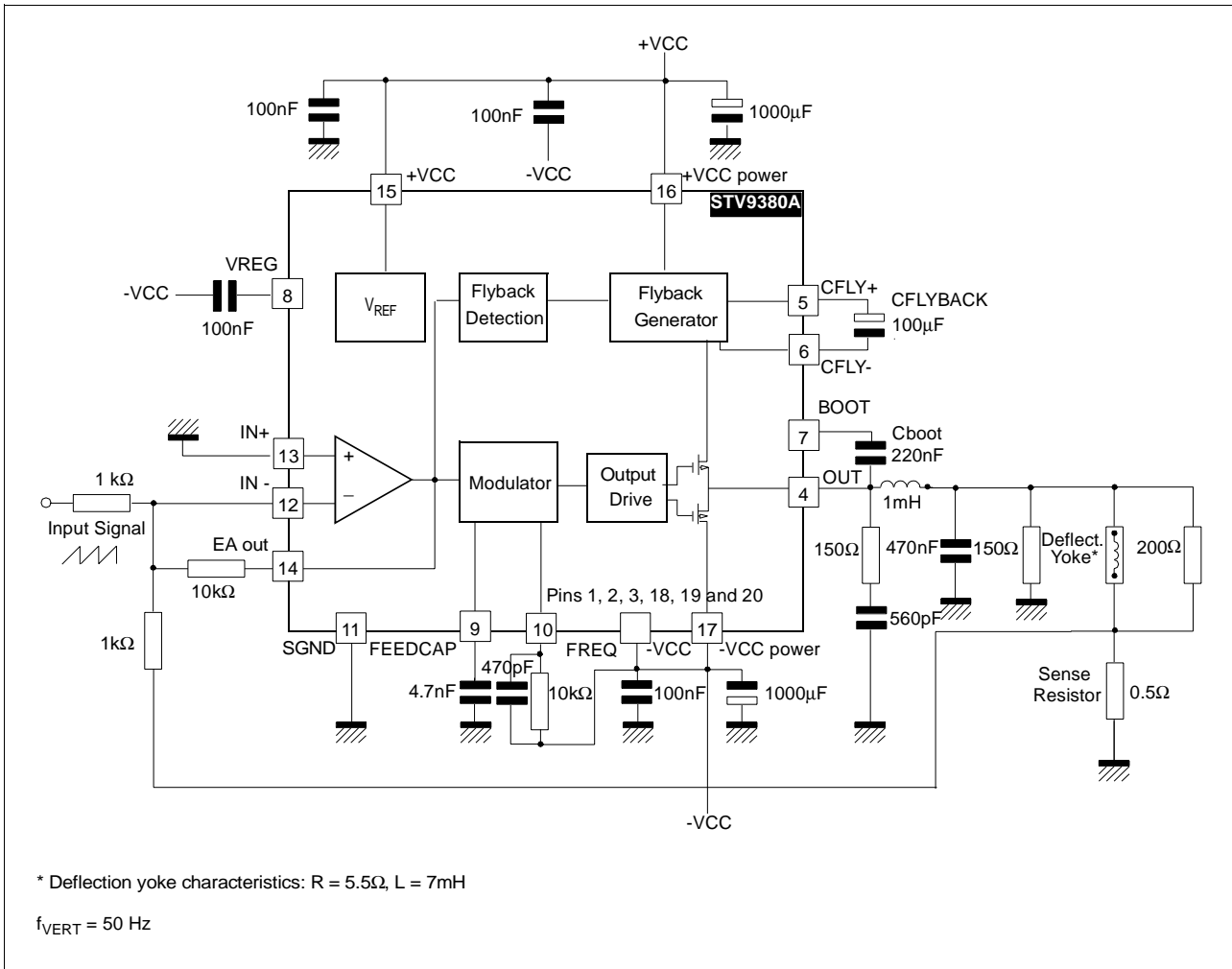
Figure 1: Test and Application Circuit Diagram
