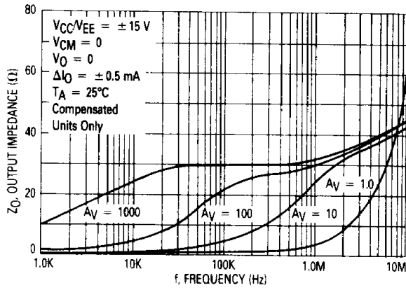
FIGURE 9 — OUTPUT IMPEDANCE versus FREQUENCY
