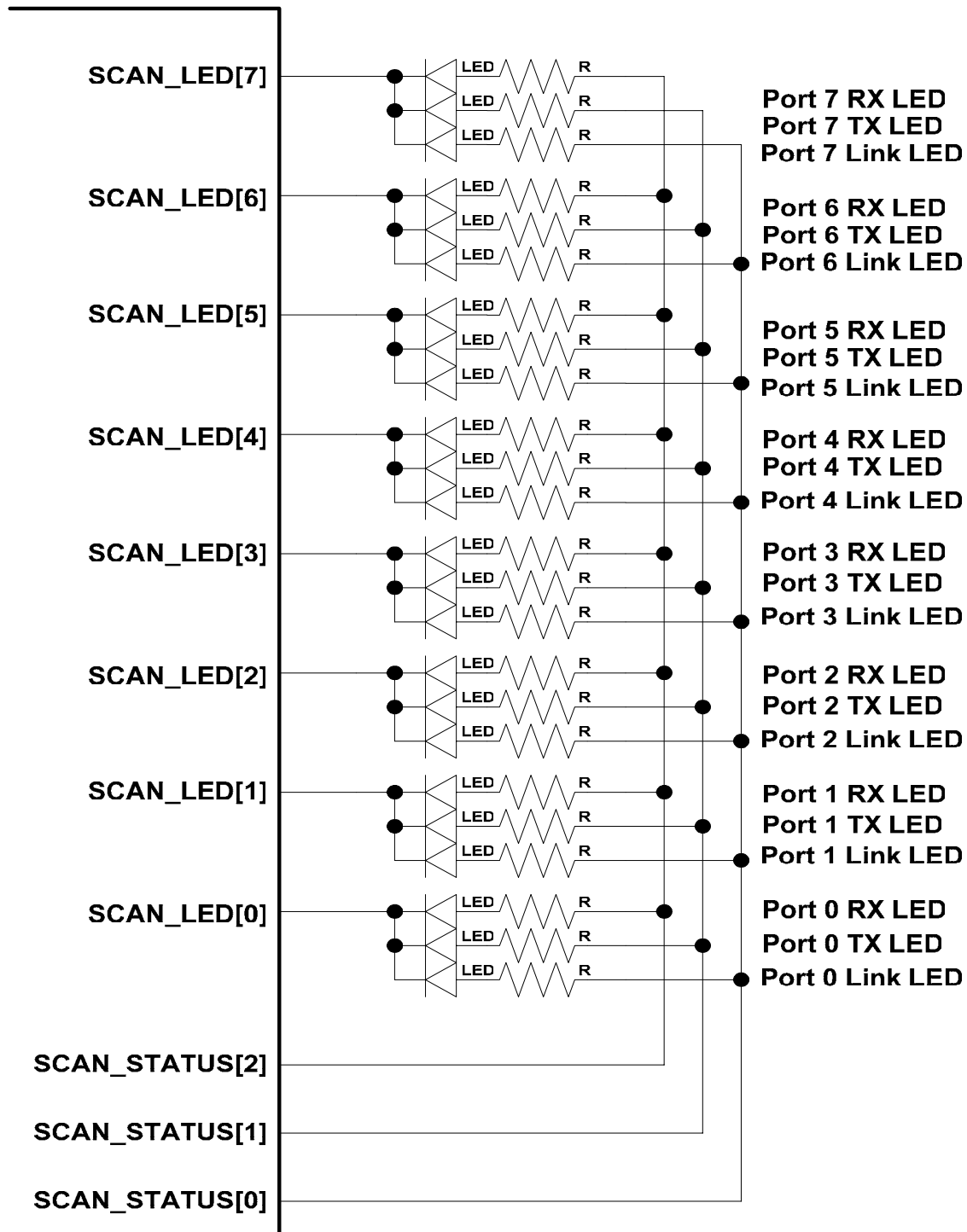
Figure 18. External Circuit for Scan LED Mode 1
