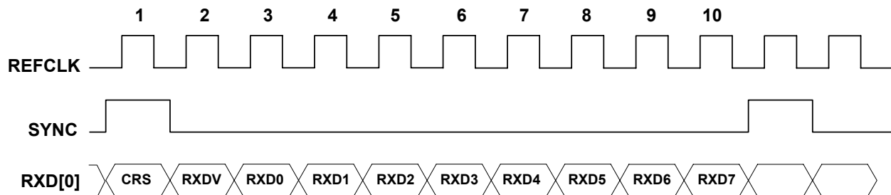
Figure 5. SMII Reception
