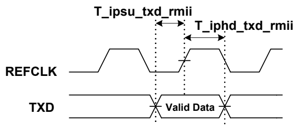
Figure 24. RMII Transmit Timing
