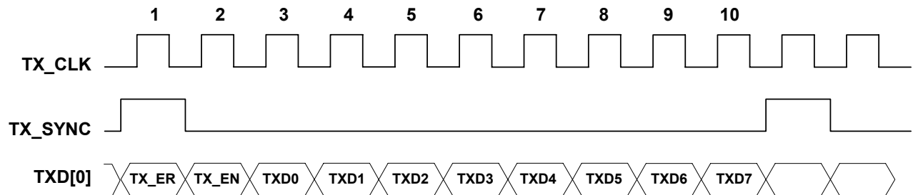
Figure 9. SS-SMII Transmission
