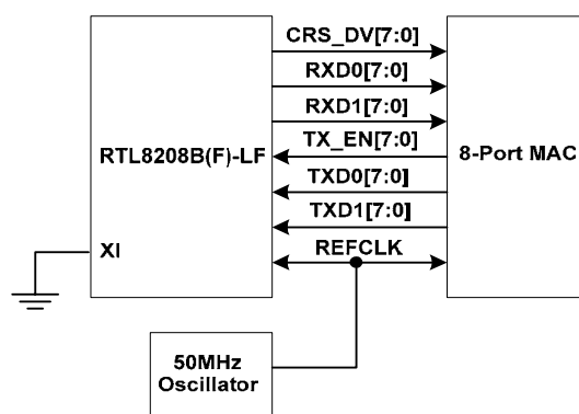
Figure 3. RMII Signal Diagram
