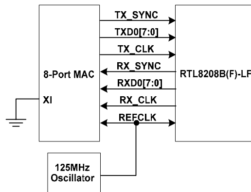
Figure 7. SS-SMII Signal Diagram
