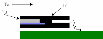
Figure 30. Cross-section of 128-Pin QFP
