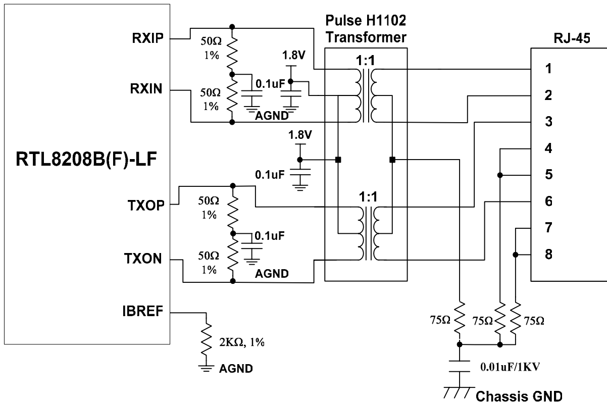
Figure 21. 10Base-T/100Base-TX Application
