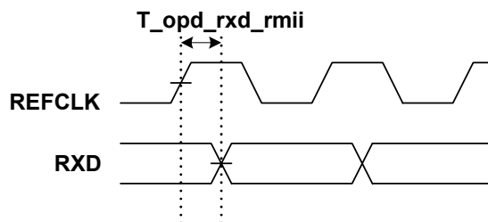
Figure 23. RMII Receive Timing
