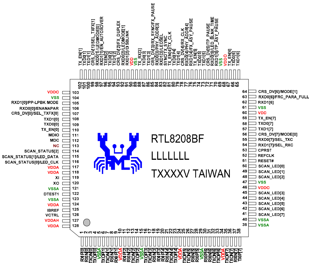
Figure 2. Pin Assignments (RTL8208BF-LF)
