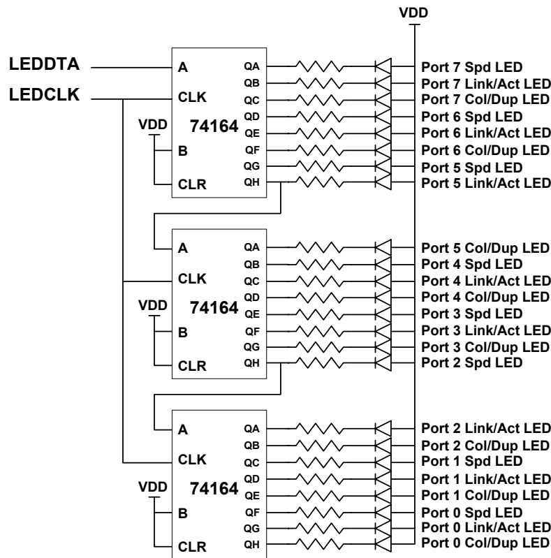
Figure 12. External Circuit for 3-Bit Serial LED Mode
