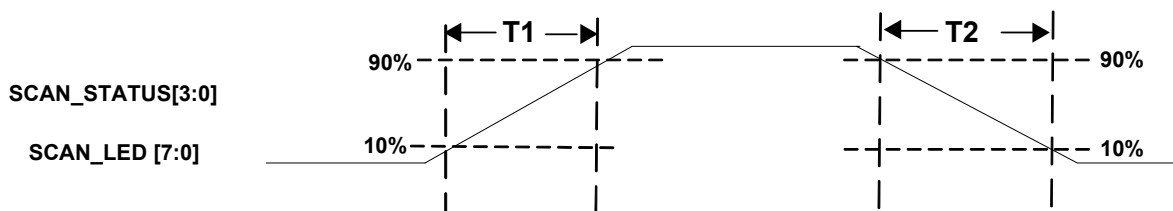
Figure 16. Rise and Fall Timing of the SCAN_STATUS and SCAN_LED Transition
