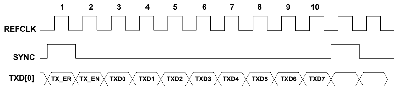
Figure 6. SMII Transmission
