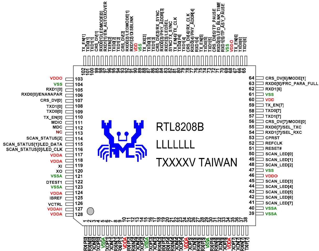
Figure 1. Pin Assignments (RTL8208B-LF)
