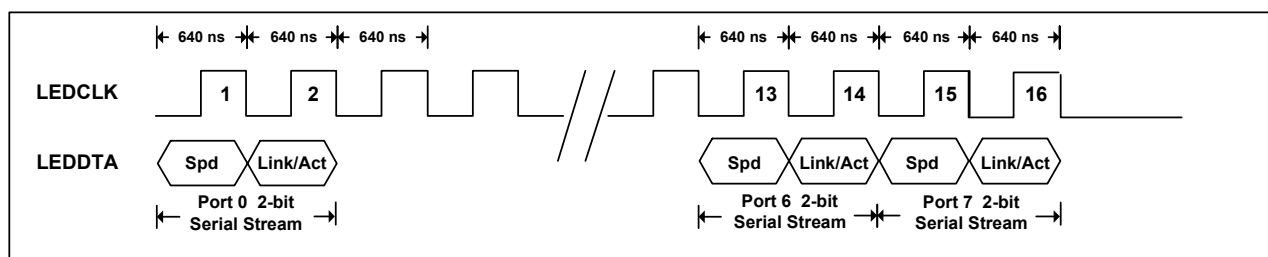
Figure 11. 2-Bit Serial Stream Mode
