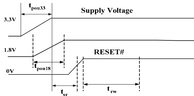
Figure 29. Power Start Up & Internal Reset Sequence
