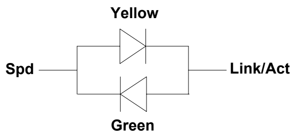
Figure 14. 3-Bit Bi-Color LED
