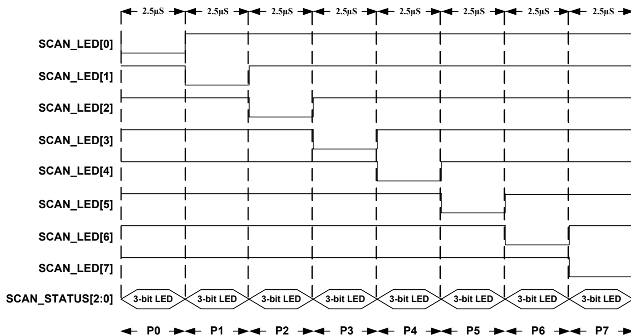
Figure 15. Scan LED Timing for Mode 0 and Mode 1
