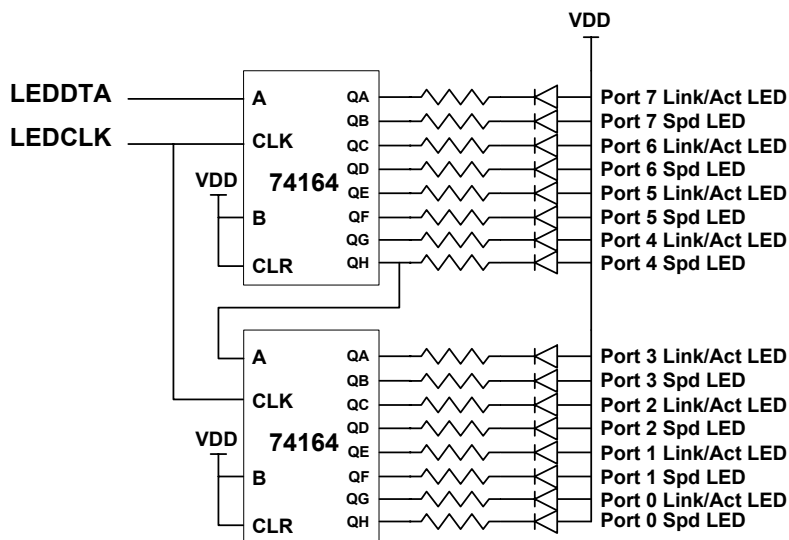
Figure 13. External Circuit for 2-Bit Serial LED Mode
