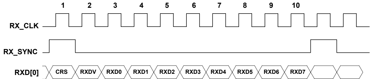
Figure 8. SS-SMII Reception
