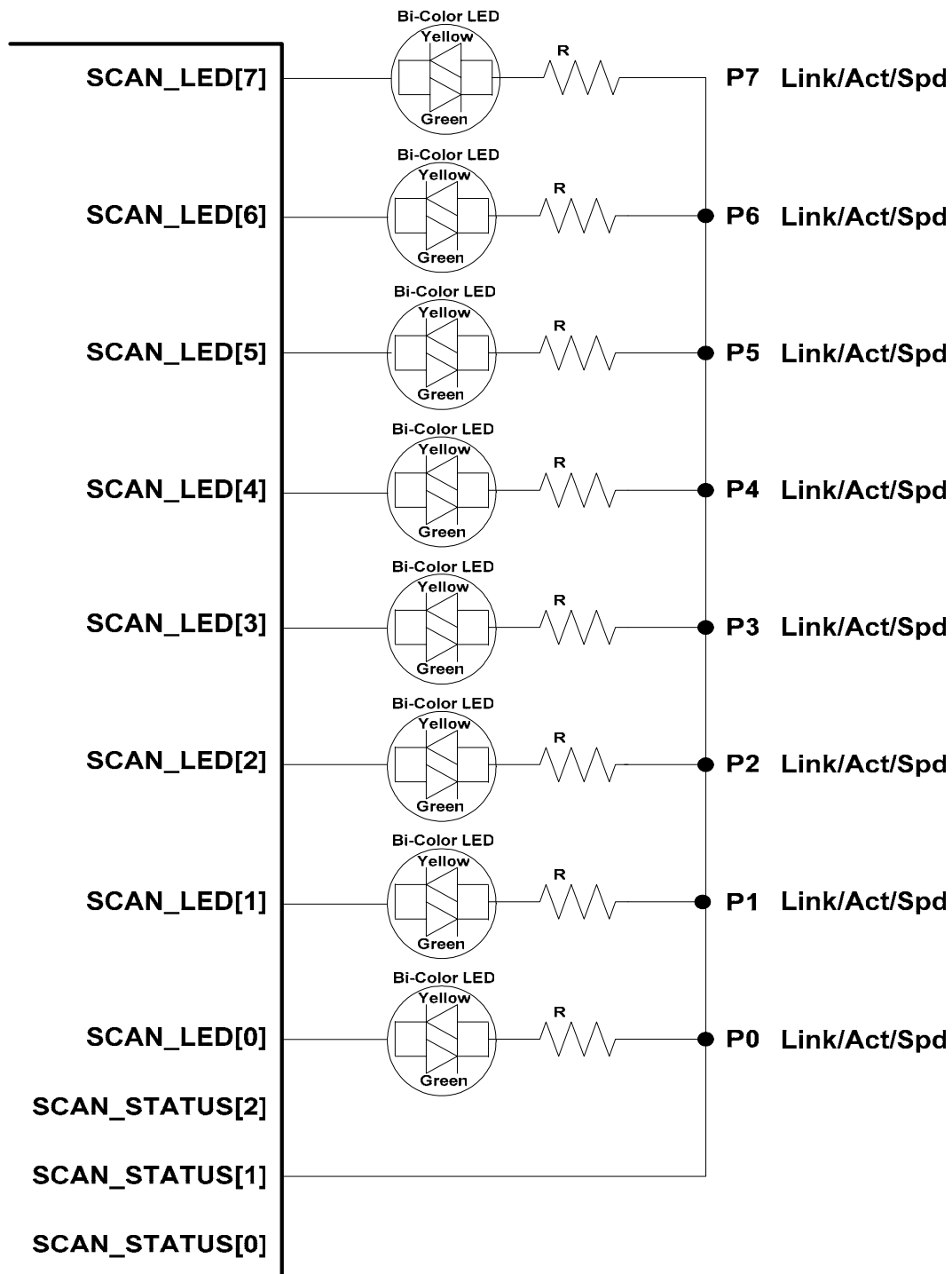
Figure 19. External Circuit for Scan LED Mode 2
