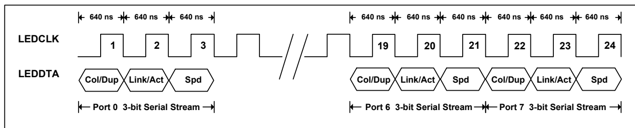
Figure 10. 3-Bit Serial Stream Mode
