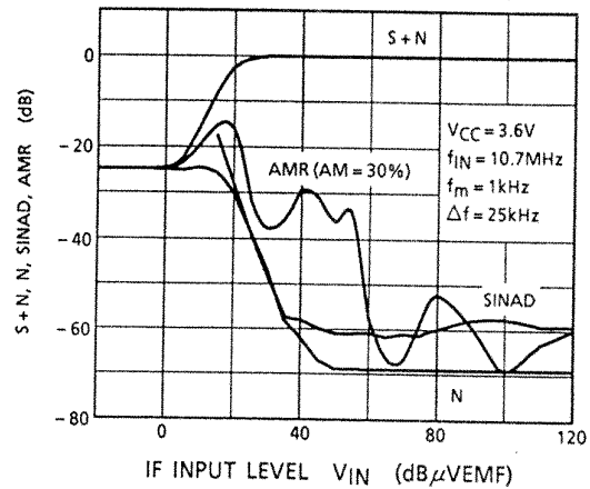
IF CHARACTERISTICS (INPUT 50Ω)
