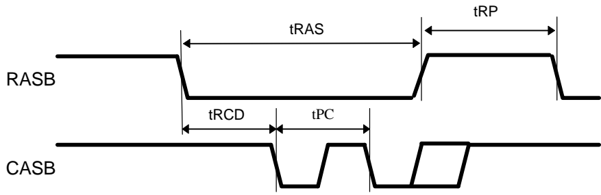
DRAM Timing
