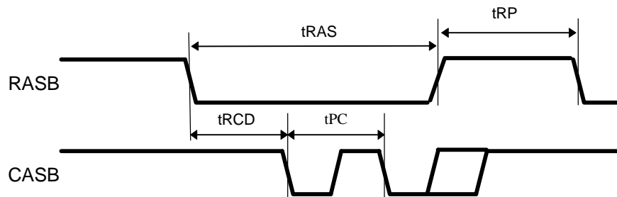
DRAM Timing
