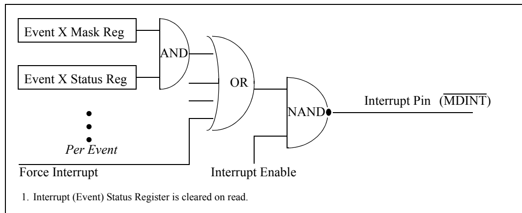
Figure 5. Interrupt Logic
