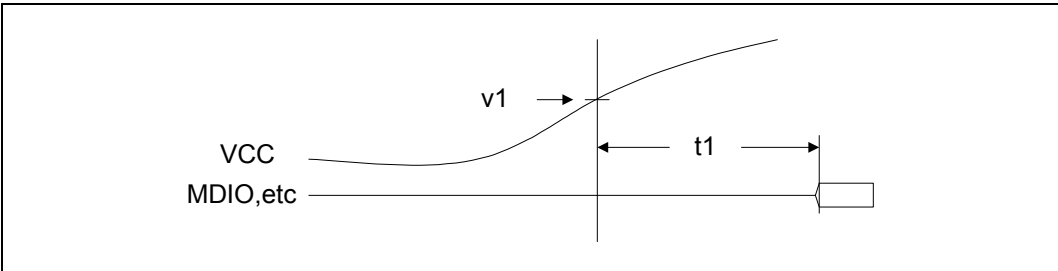
Figure 34. Power-Up Timing
