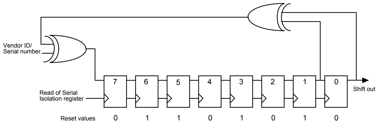
Figure 3. Checksum LFSR
