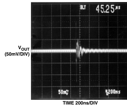
TPC 17. Digital Feedthrough vs. Time
