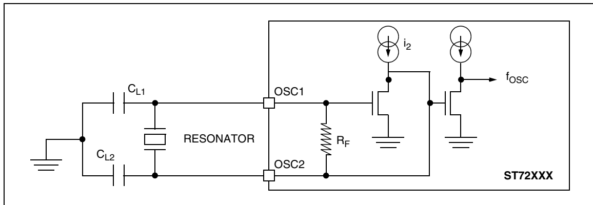
Figure 67. Application with a Crystal Resonator
