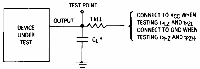
Figure 6. Test Circuit
