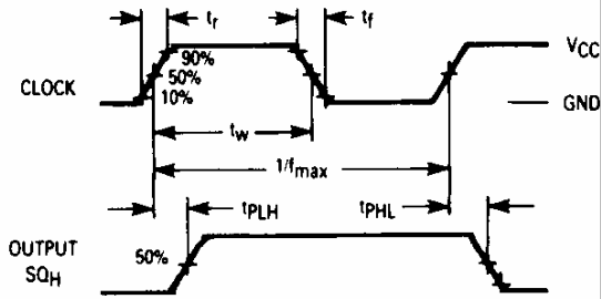
Figure 1. Switching Waveforms
