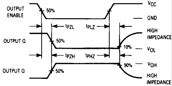
Figure 3. Switching Waveforms
