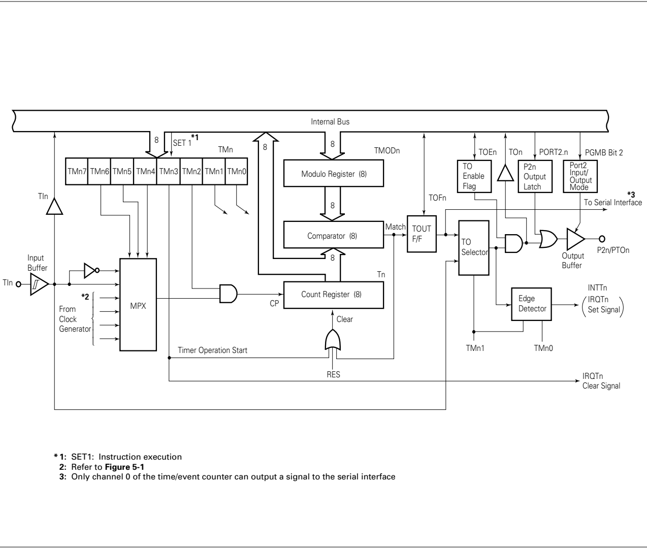
Figure 5-4 Block Diagram of Timer/Event Counter (n=0, 1)
