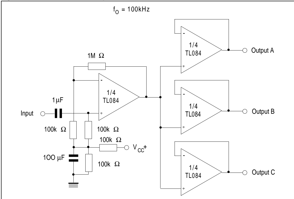
Figure 21. Audio distribution amplifier
