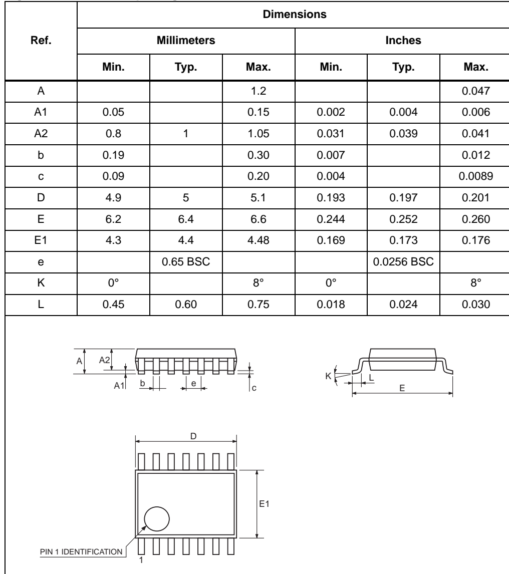
Figure 25. TSSOP14 package mechanical data
