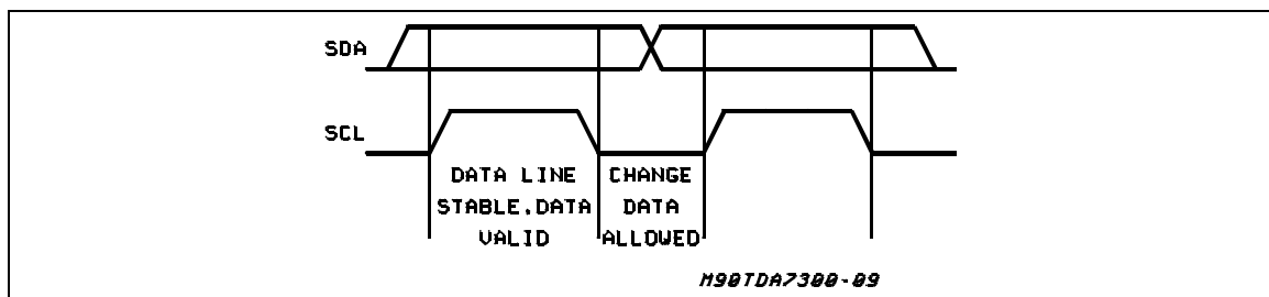
Figure 17: Data Validity on the I 2 C BUS
