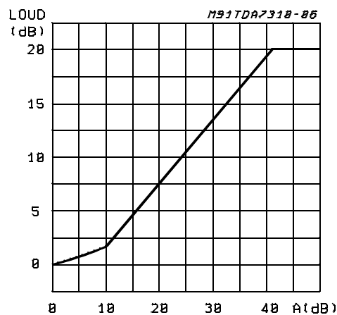
Figure 1: Loudness vs. Volume Attenuation
