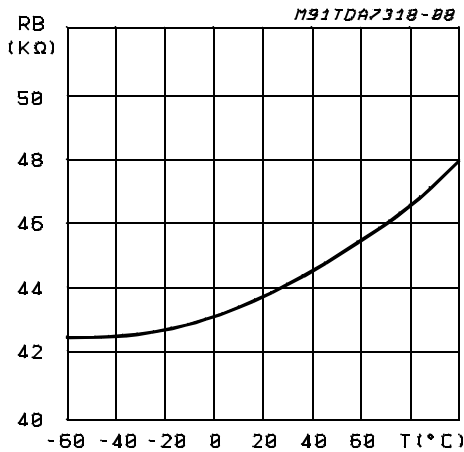
Figure 15: Bass Resistance vs. Temperature
