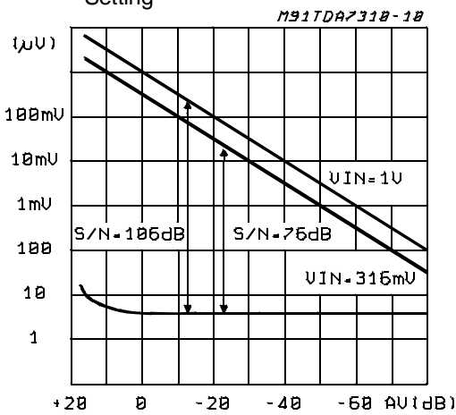
Figure 5: Signal to Noise Ratio vs. Volume Setting
