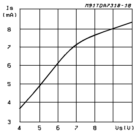
Figure 13: Quiescent Current vs. Supply Voltage
