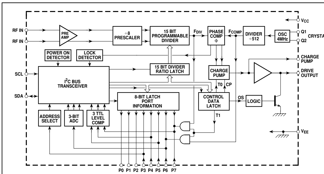
Fig. 2 Block diagram. (Ports P0-P2 not present on SP5510S)
