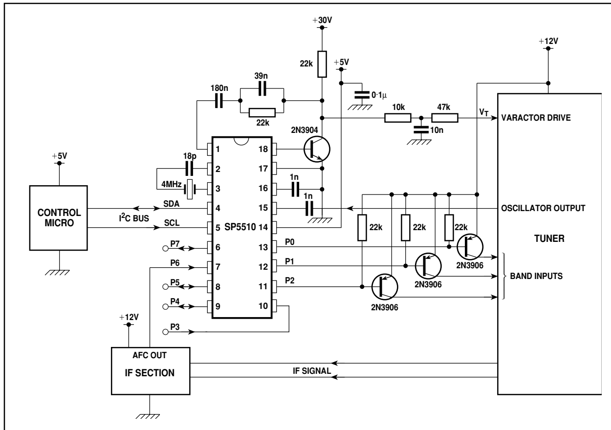
Fig. 4 Typical application
