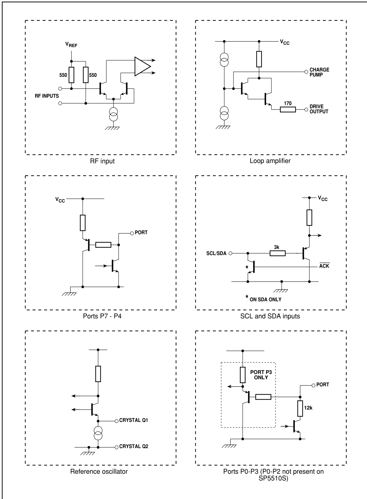
Fig. 6 SP5510 input/output interface circuits
