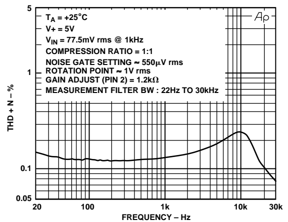
Figure 8. THD+N (%) vs. Frequency (Hz)
