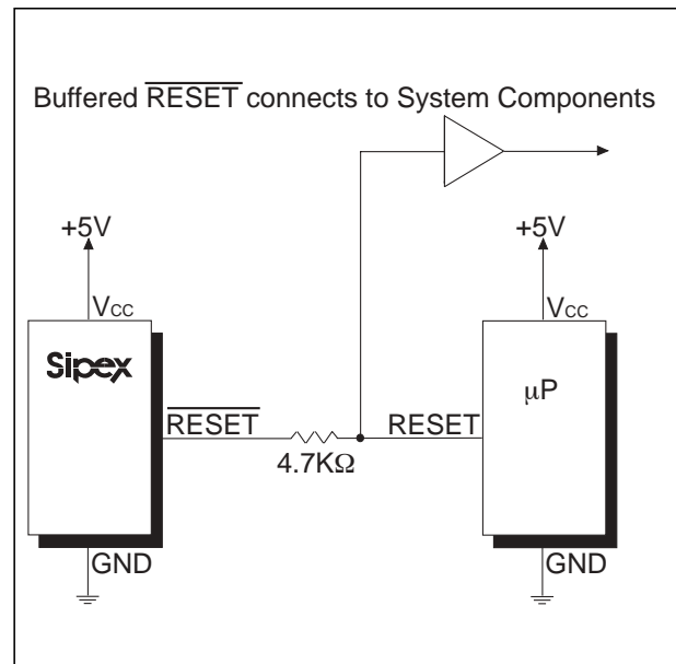
Figure 20. Interfacing to Microprocessors with Bidirectional \overline{RESET} I/O
