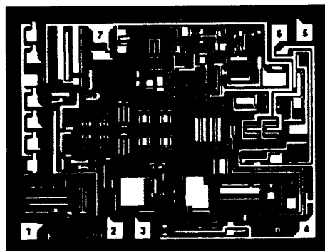
DIE SIZE 0.103 × 0.074 inch, 7922 sq. mils (2.62 × 1.88mm, 4.92 sq. mm)
