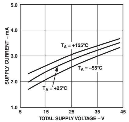
TPC 9. Supply Current vs. Supply Voltage
