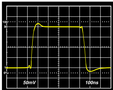
Small Signal Response R_L = 2\text{ k}\Omega , V_S = \pm 15\text{ V} , A_V = +1
