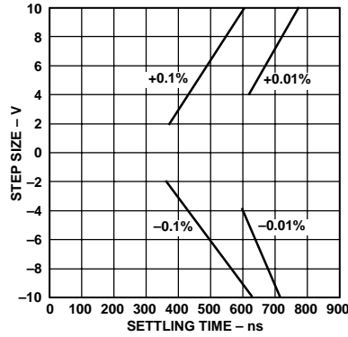
Settling Time vs. Step Size
