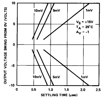
SETTLING TIME
