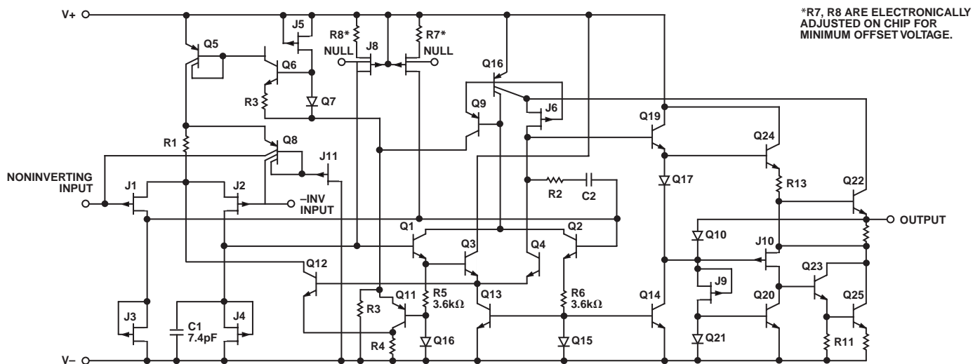
Figure 1. Simplified Schematic
