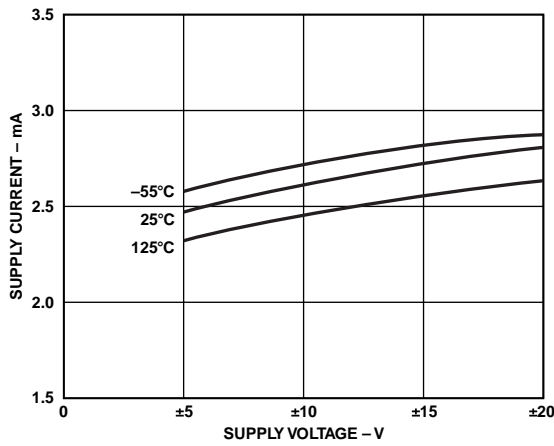
TPC 14. OP15 Supply Current vs. Supply Voltage
