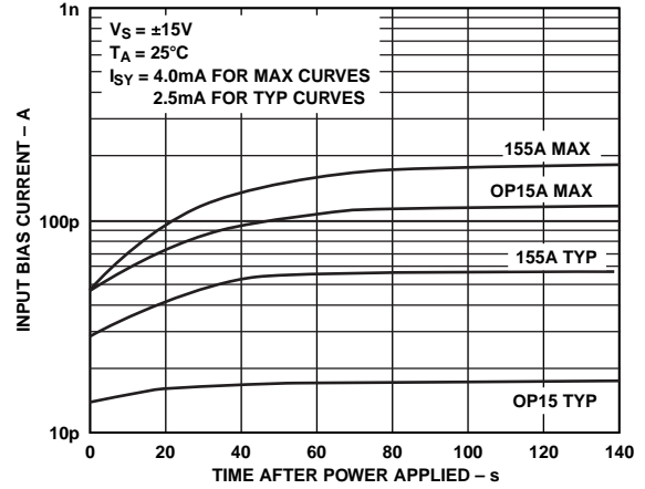
TPC 10. OP15 Bias Current vs. Time in Free Air
