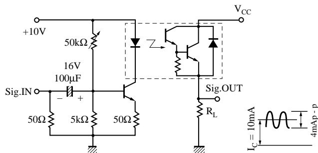
Measurement circuit of frequency characteristics
