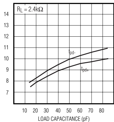
RESPONSE TIME vs. LOAD CAPACITANCE (5mV OVERDRIVE)
