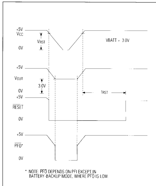
Figure 2. Timing Diagram
