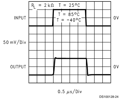
Non-Inverting Small Signal Pulse Response
