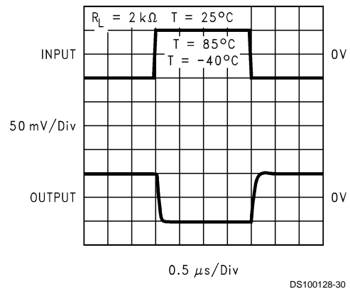
Inverting Small Signal Pulse Response
