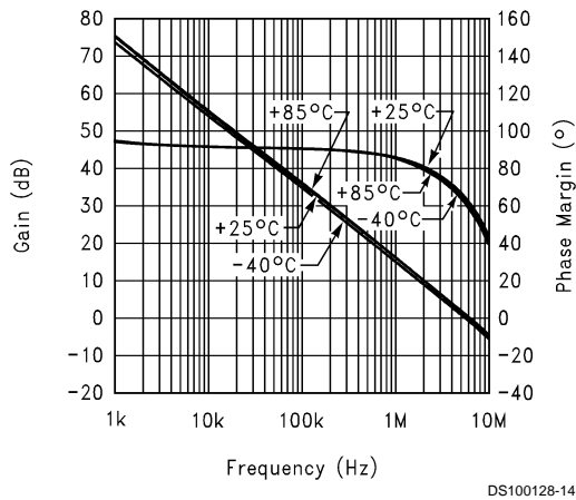
Gain and Phase Margin vs. Frequency (Temp. = 25, -40, 85^\circ C, R_L = 10k\Omega) 5V
