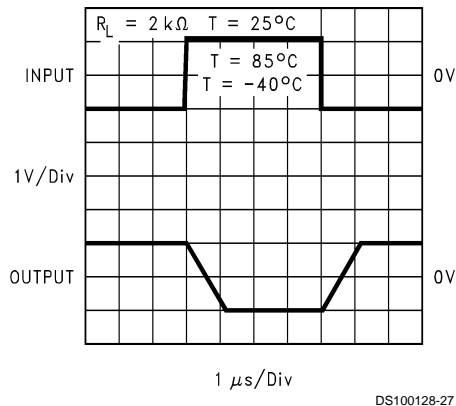
Inverting Large Signal Pulse Response
