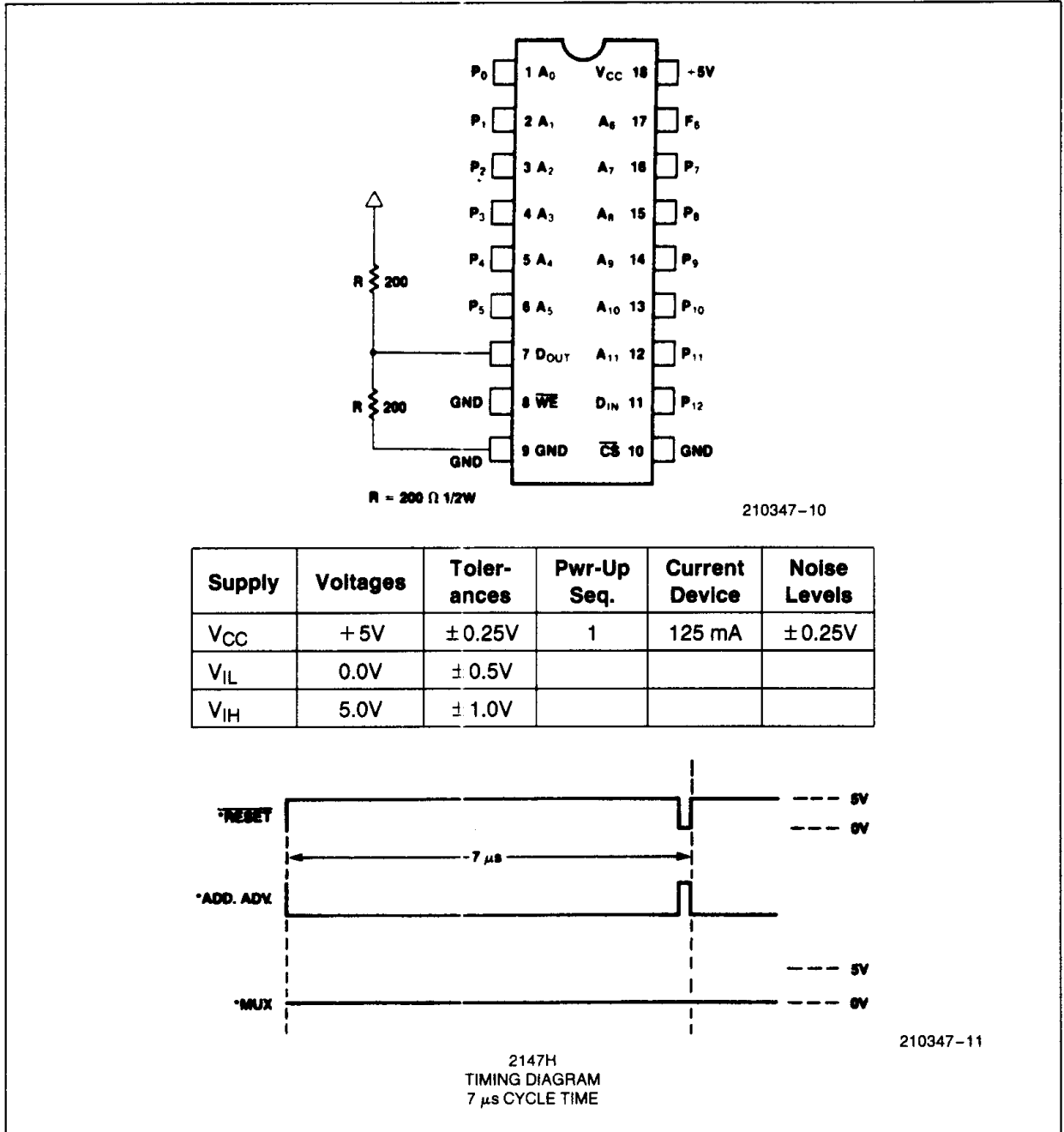
Figure 3. 2147H Burn-In Configuration
