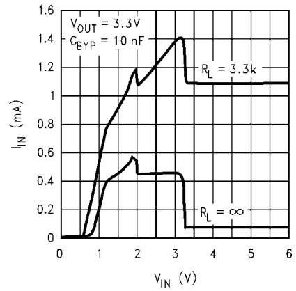
Input Current vs Pin
