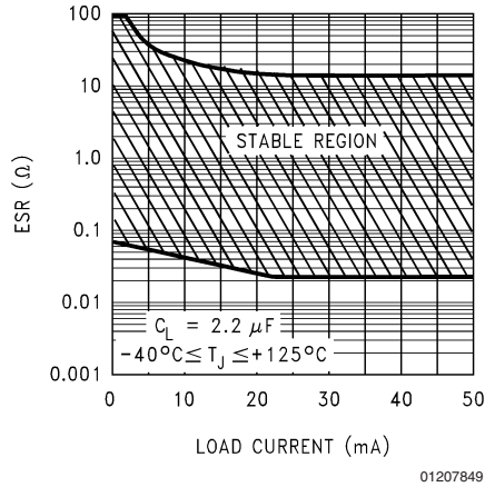
FIGURE 2. 2.2 μF ESR Range
