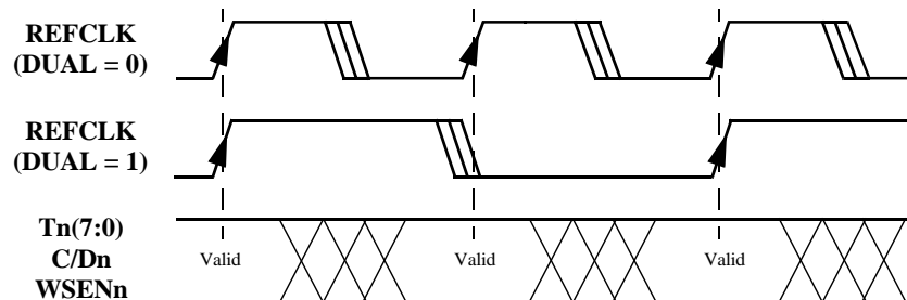
Figure 2: Transmit Timing, TMODE(2:0) = 000
