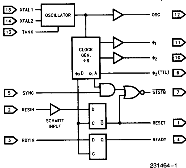
Figure 1. Block Diagram
