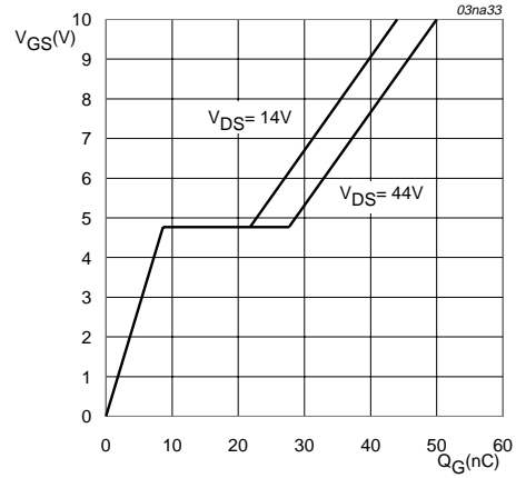
T_j = 25^\circ\text{C}; I_D = 25\text{ A} Fig 14. Turn-on gate charge characteristics; typical values.
