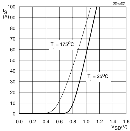
V_{GS} = 0\text{ V} Fig 15. Reverse diode current; typical values.
