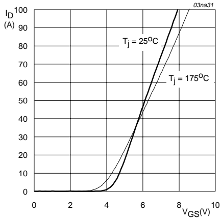
V_{DS} = 25\text{ V} Fig 13. Transfer characteristics; typical values.
