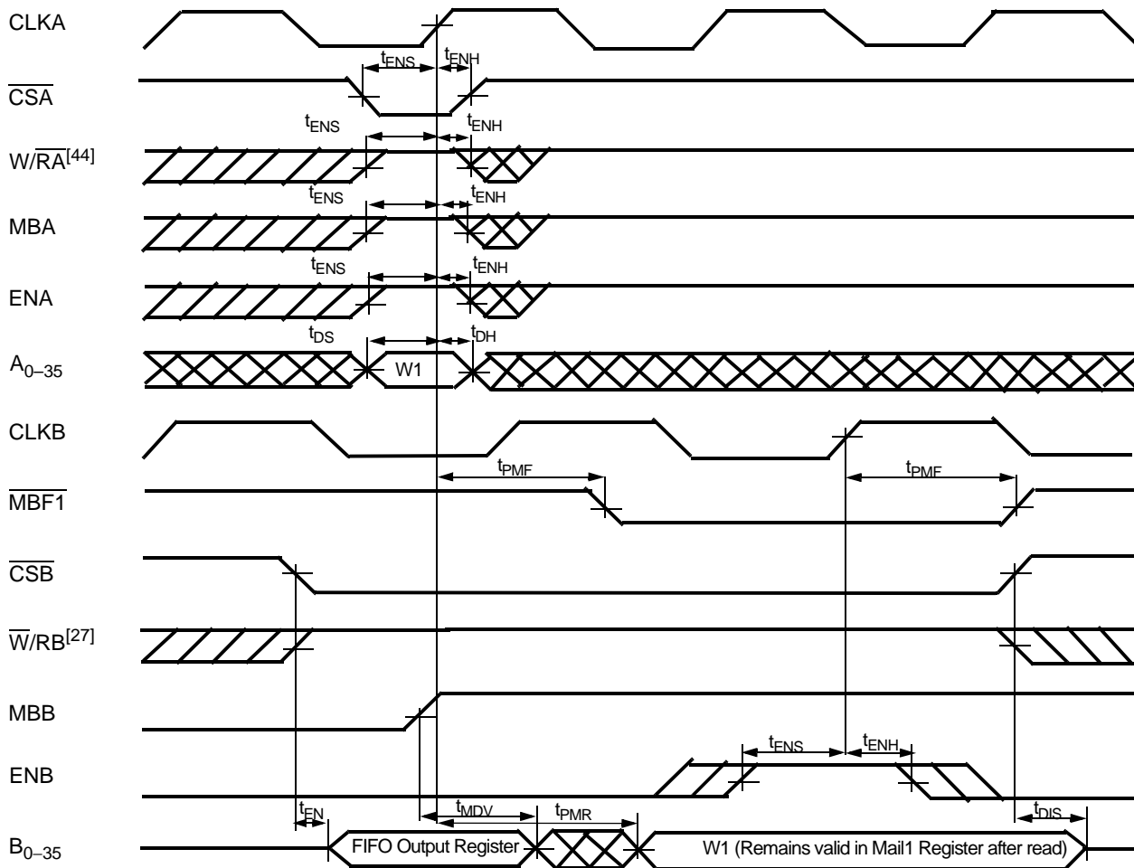
Timing for Mail1 Register and \overline{\text{MBF1}} Flag (CY Standard and FWFT Modes) [43,45]
