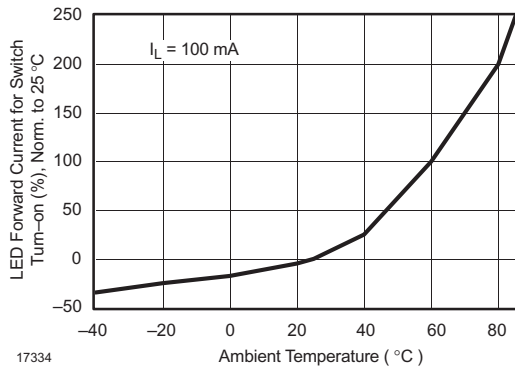
Figure 3. LED Current for Switch Turn-on vs. Temperature
