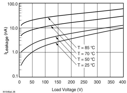
Figure 6. Leakage Current vs. Applied Voltage
