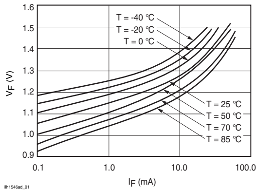
Figure 2. LED Voltage vs. Temperature
