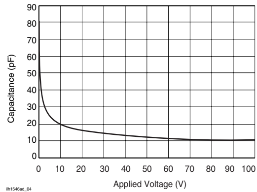
Figure 5. Switch Capacitance vs. Applied Voltage
