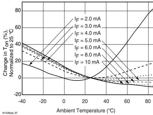
Figure 7. Turn-on Time vs. Temperature
