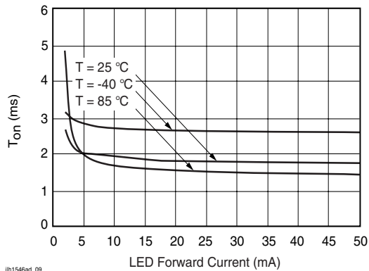
Figure 9. Turn-on Time vs. LED Current
