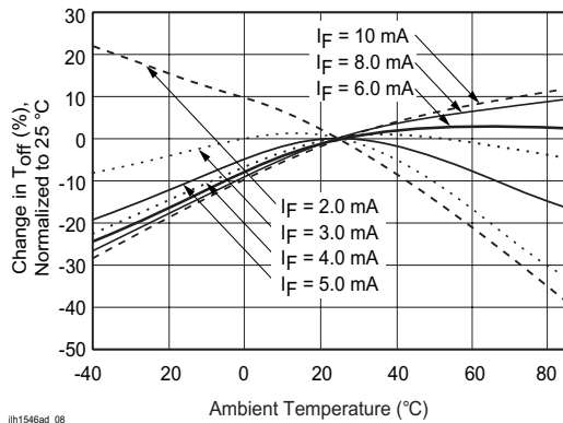
Figure 8. Turn-off Time vs. Temperature
