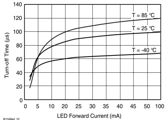
Figure 10. Turn-off Time vs. LED Current
