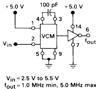
FIGURE 3 — VOLTAGE-CONTROLLED MULTIVIBRATOR
