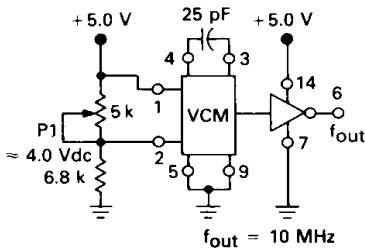
FIGURE 1 — ASTABLE MULTIVIBRATOR
