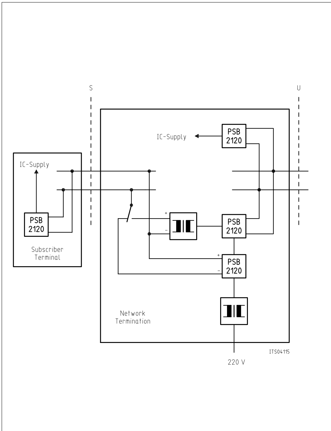
Figure 3 IRPC in ISDN-Concept
