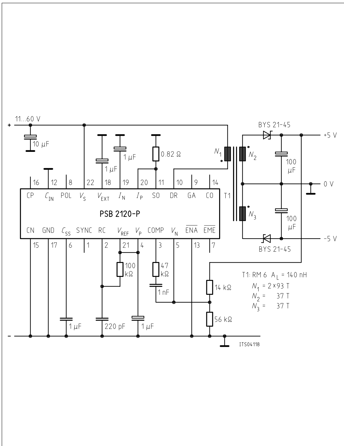
Figure 5 PSB 2120 Minimum Configuration
