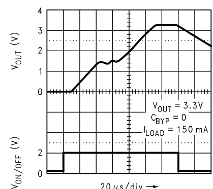
Turn-On Time
