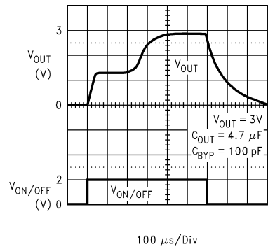
Turn-ON Waveform
