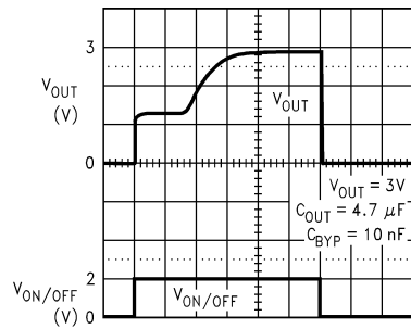
10 \text{ms}/\text{Div} DS012679-52
