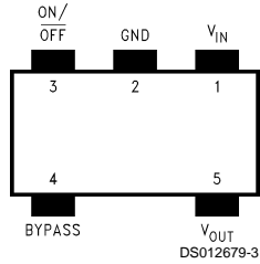
5-Lead Small Outline Package (M5)
