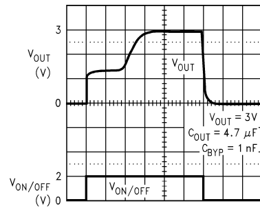
1 \text{ms}/\text{Div} DS012679-51
