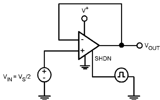
FIGURE 4. Turn-off Time
