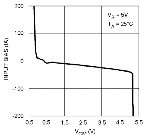
FIGURE 7. Input Bias Current vs. V_{CM}
