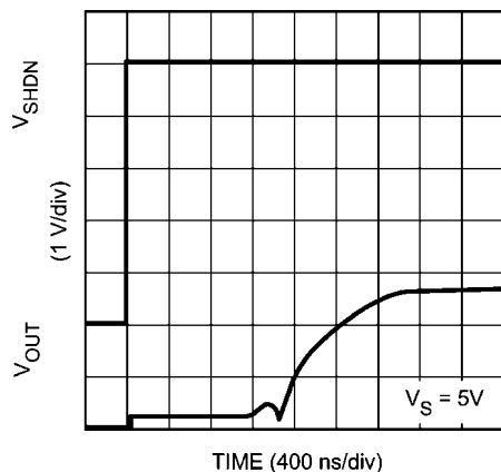
FIGURE 3. Turn-on Time
