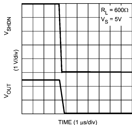
FIGURE 4. Turn-off Time
