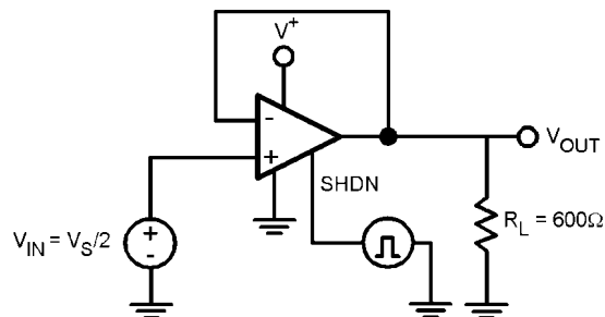
FIGURE 6. Turn-off Time
