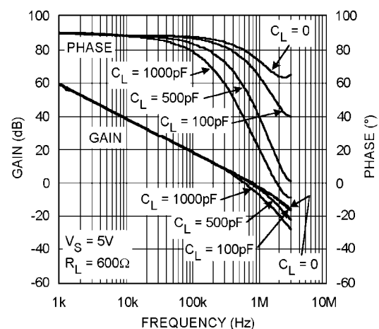
Gain and Phase vs. C_L
