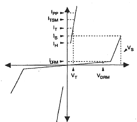
FIGURE 7 V - I CHARACTERISTICS CURVE
