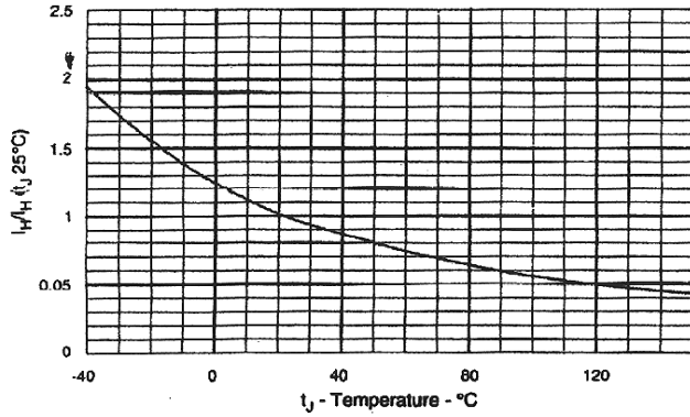
FIGURE 4 TYPICAL HOLDING CURRENT VS JUNCTION TEMPERATURE
